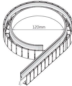
Min. Bending Diameter (Toothed Side outwards)
